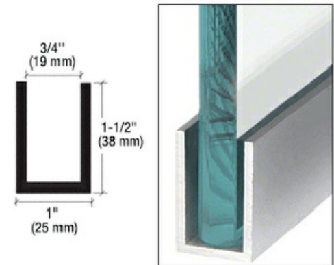
CRL Satin Anodized Wet Glaze 1-1/2" Deep U-Channel
