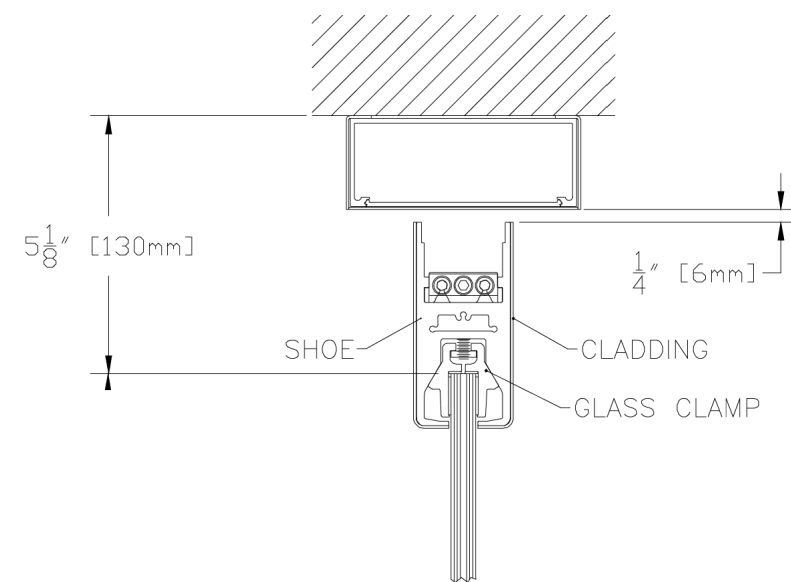
CRL Satin Anodized 4-1/2" x 36" Single Door Header
