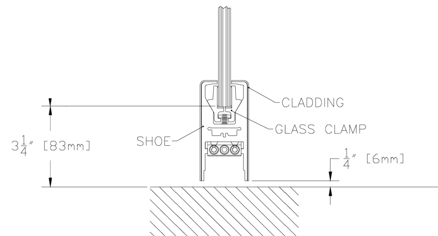
CRL Satin Anodized 1/2" Glass 4" Square Door Rail Without Lock - 35-3/4" Length
