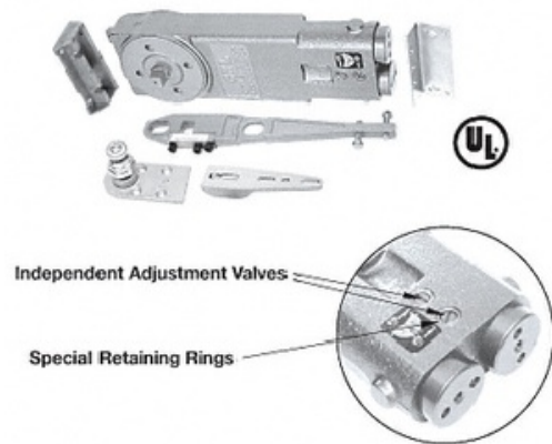
CRL Medium Duty 90° Hold Open Overhead Concealed Closer with S-Side-Load Hardware Package
